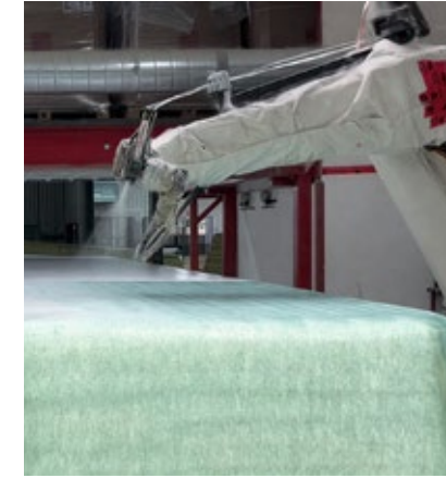
3 Barrier Coat Application
